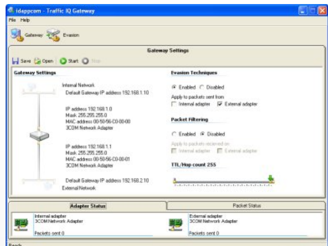
Traffic IQ Gateway - Inline Advanced Evasion Techniques
